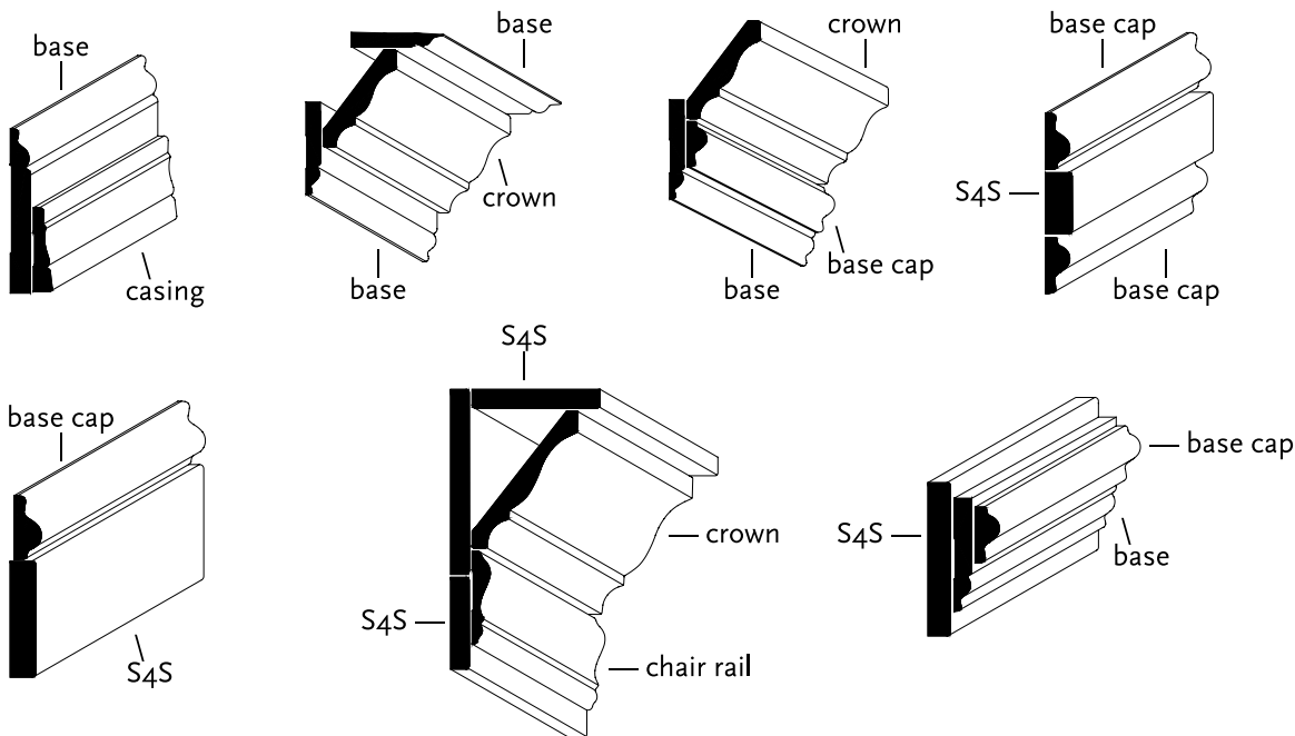
BASE MOULDING
